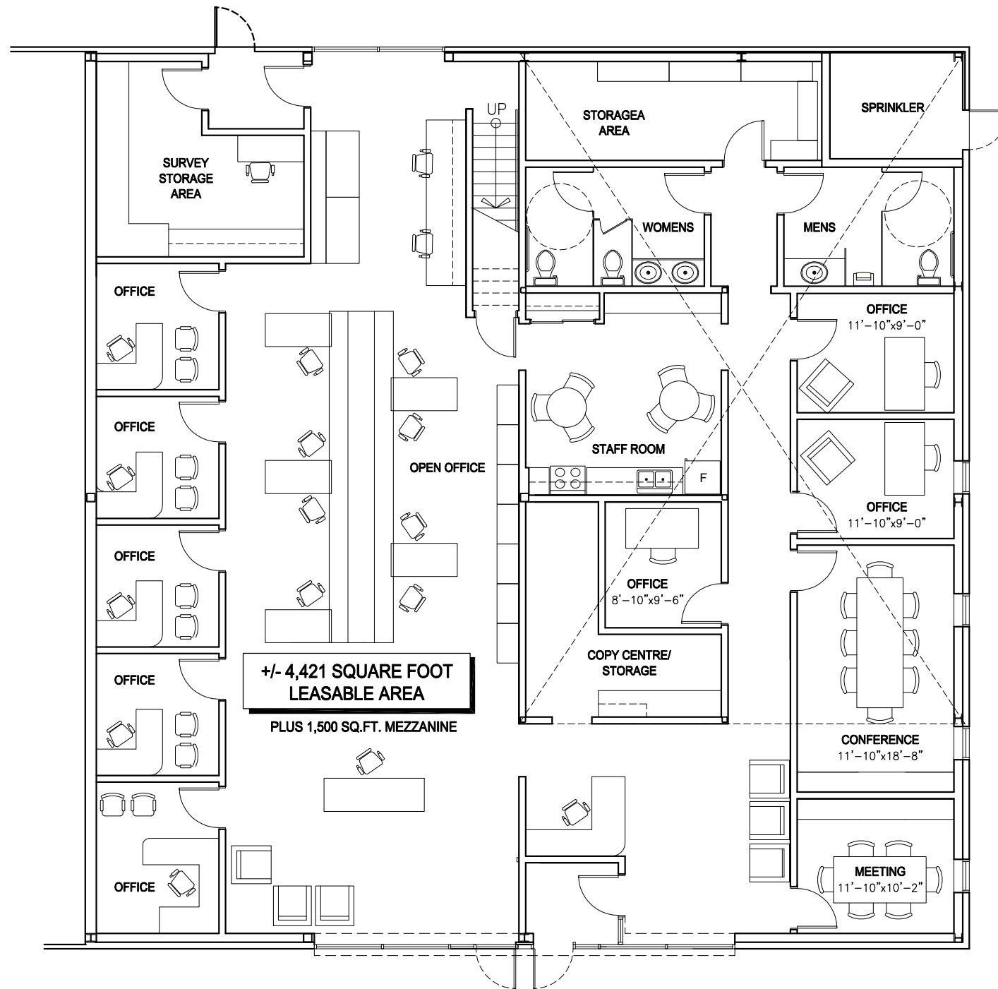
FLOOR PLAN
